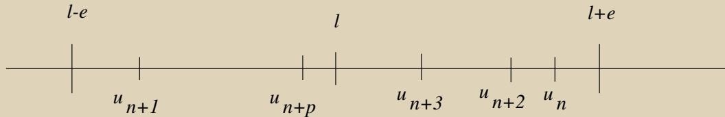
FIGURE C.1.2 – convergence de la suite
